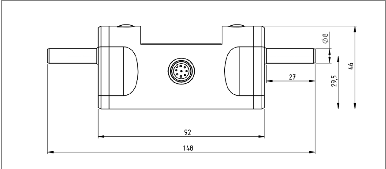
Figure 1: Dimensions SONOFLOW IL.52 V2.0 – Side view
